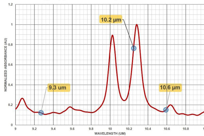
Polypropylene Film Absorption Characteristics
