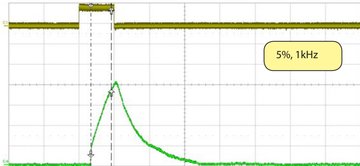
Figure 4-7 Representative output energy profile-5% duty cycle, 1kHz, time base 50 \mu s/Div.
