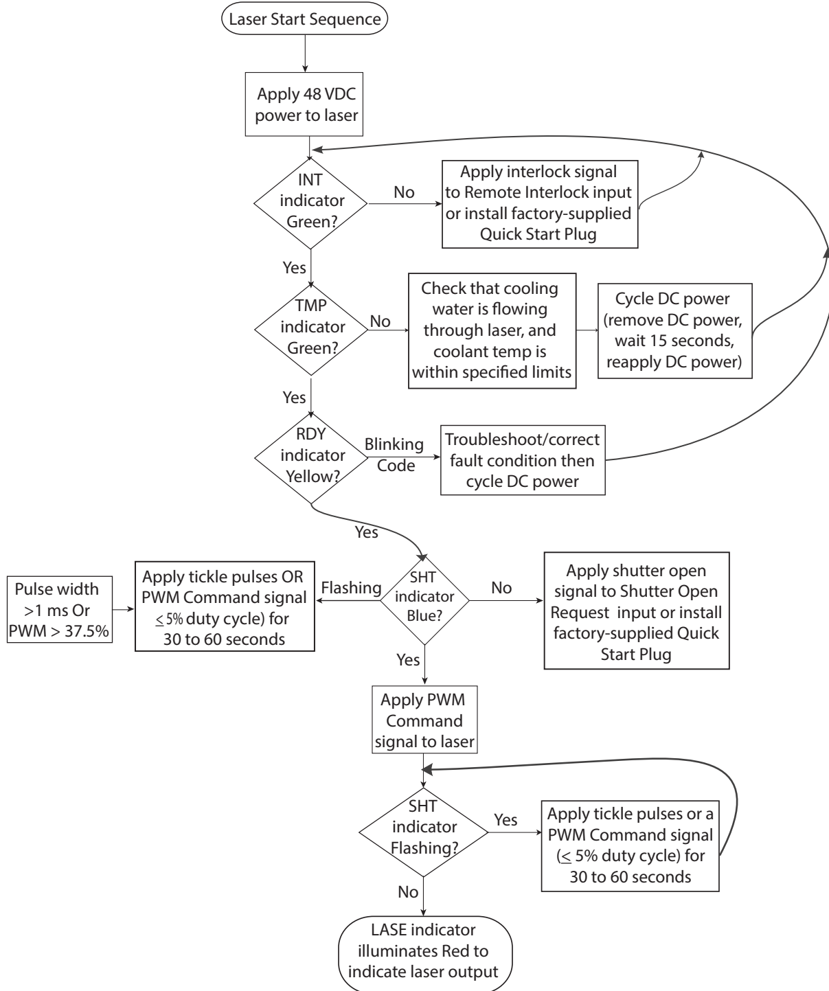
Figure 5-1 P400 operational flowchart.
