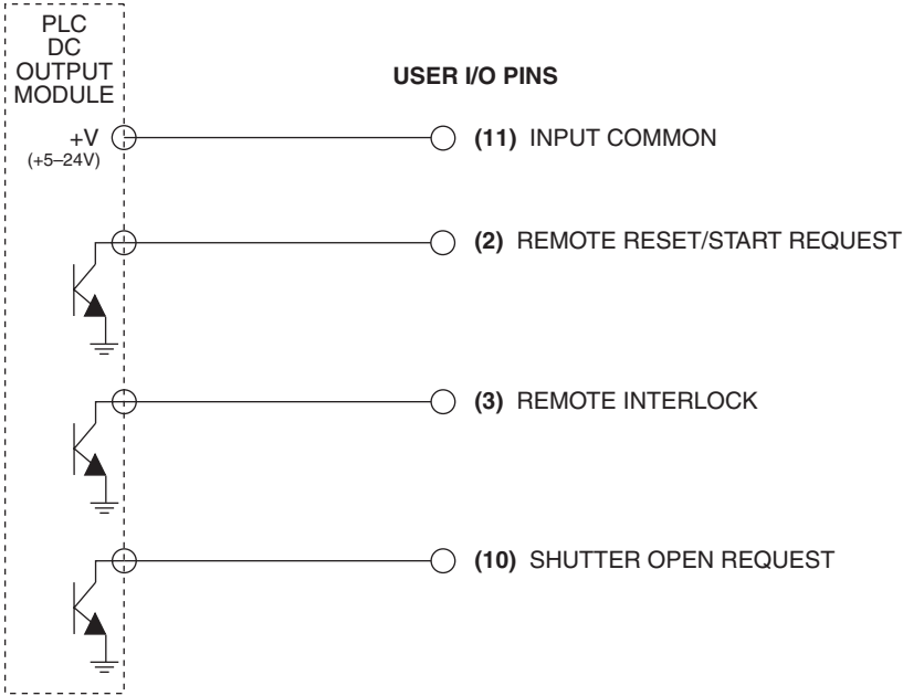
Figure 4-30 Multiple PLC driven inputs.
