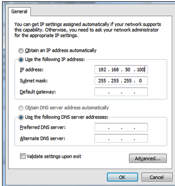
Figure 4-41 Internet Protocol (TCP/IP) Properties dialog.
