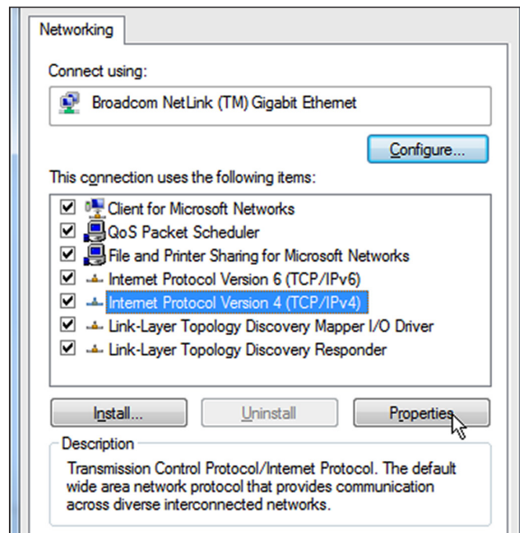
Figure 4-40 Local Area Connection Properties dialog.
