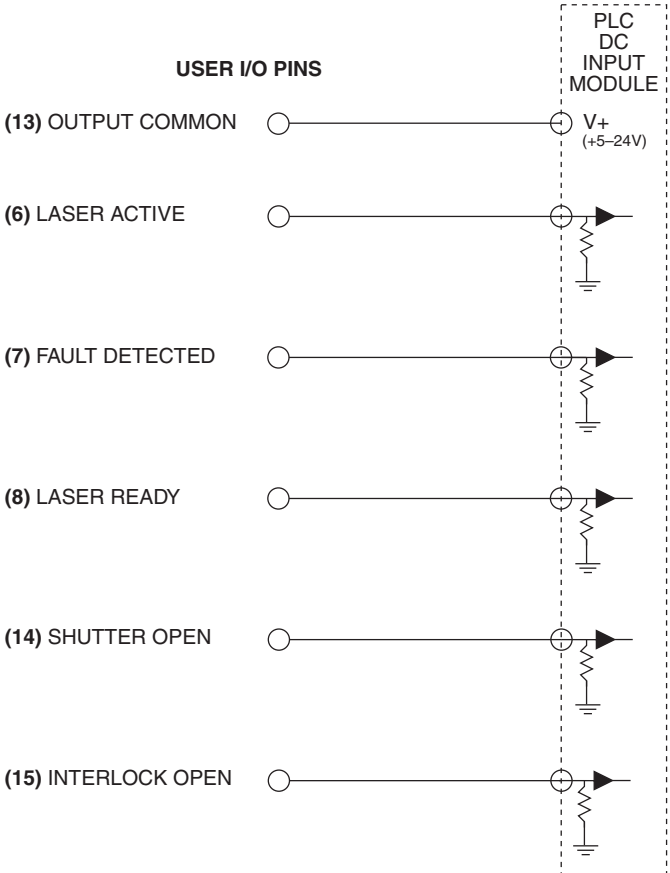
Figure 4-33 P400 output driving PLC input module.
