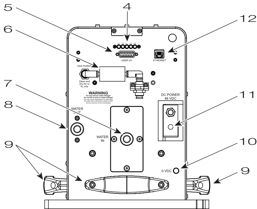
Figure 3-2 Pulstar p400 rear panel controls and indicators.
