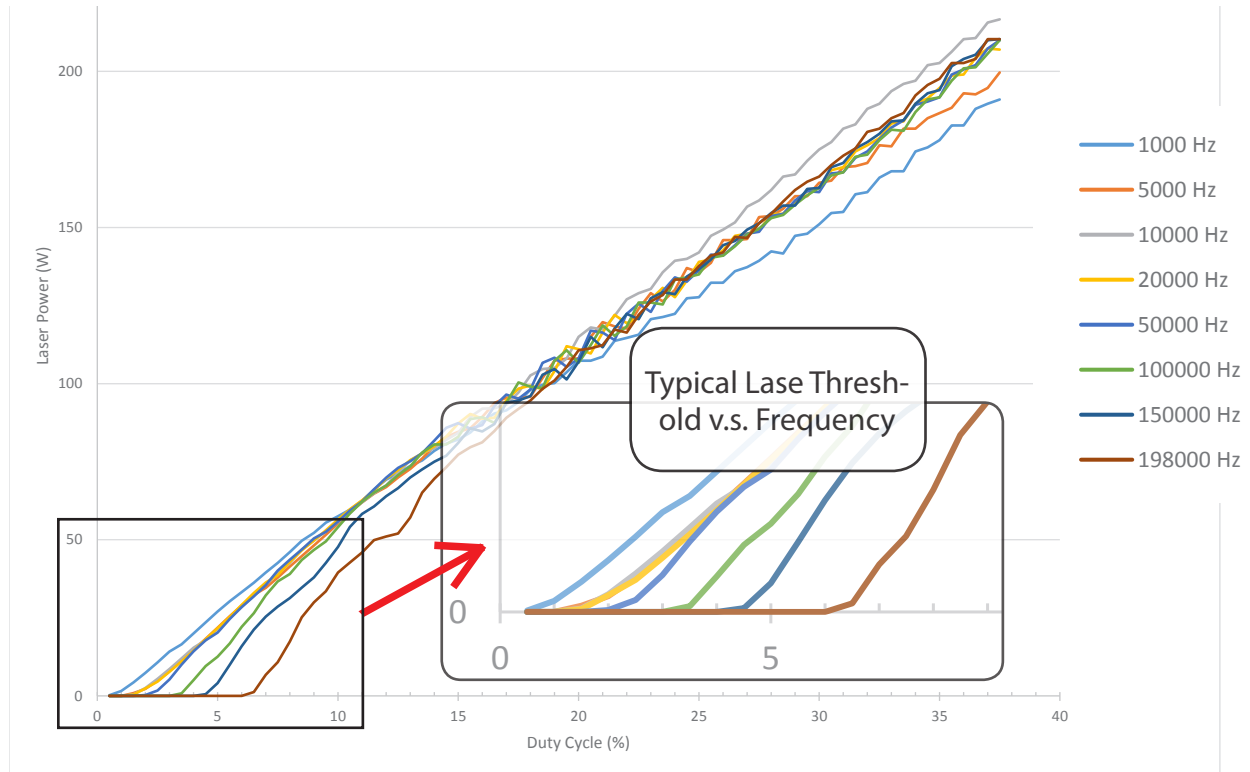
Figure 4-5 Typical power curve.
