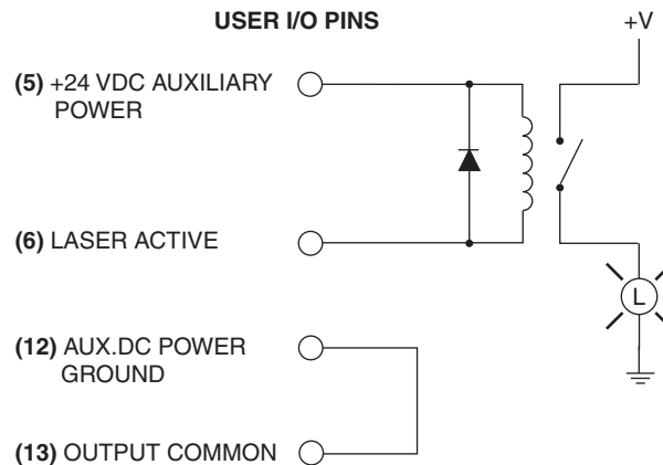
Figure 4-32 P400 output driving relay.
