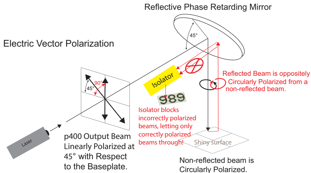
Figure 4-3 Converting 45^\circ linear polarization to circular polarization.
