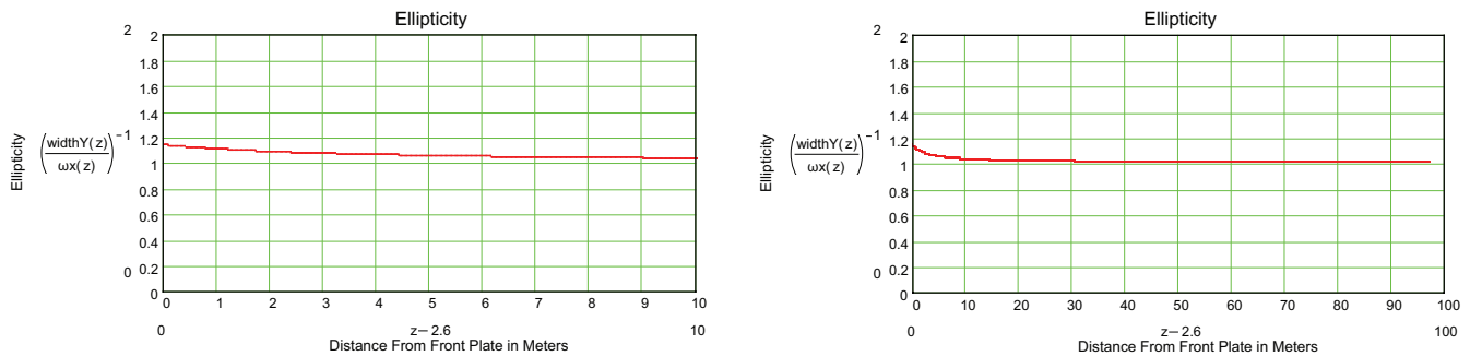
Figure 4-2 P400 beam ellipticity.
