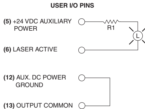
Figure 4-31 P400 output driving warning lamp.
