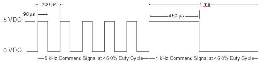
Figure 4-4 PWM command signal wave form (above) and Quasai Continuous Wave (QCW) explanation.
