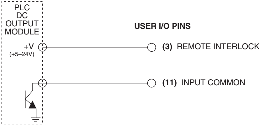
Figure 4-29 PLC driven interlock signal.
