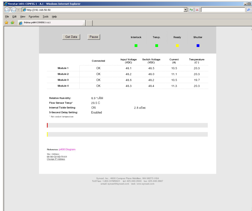
Figure 4-34 P400 home page.
