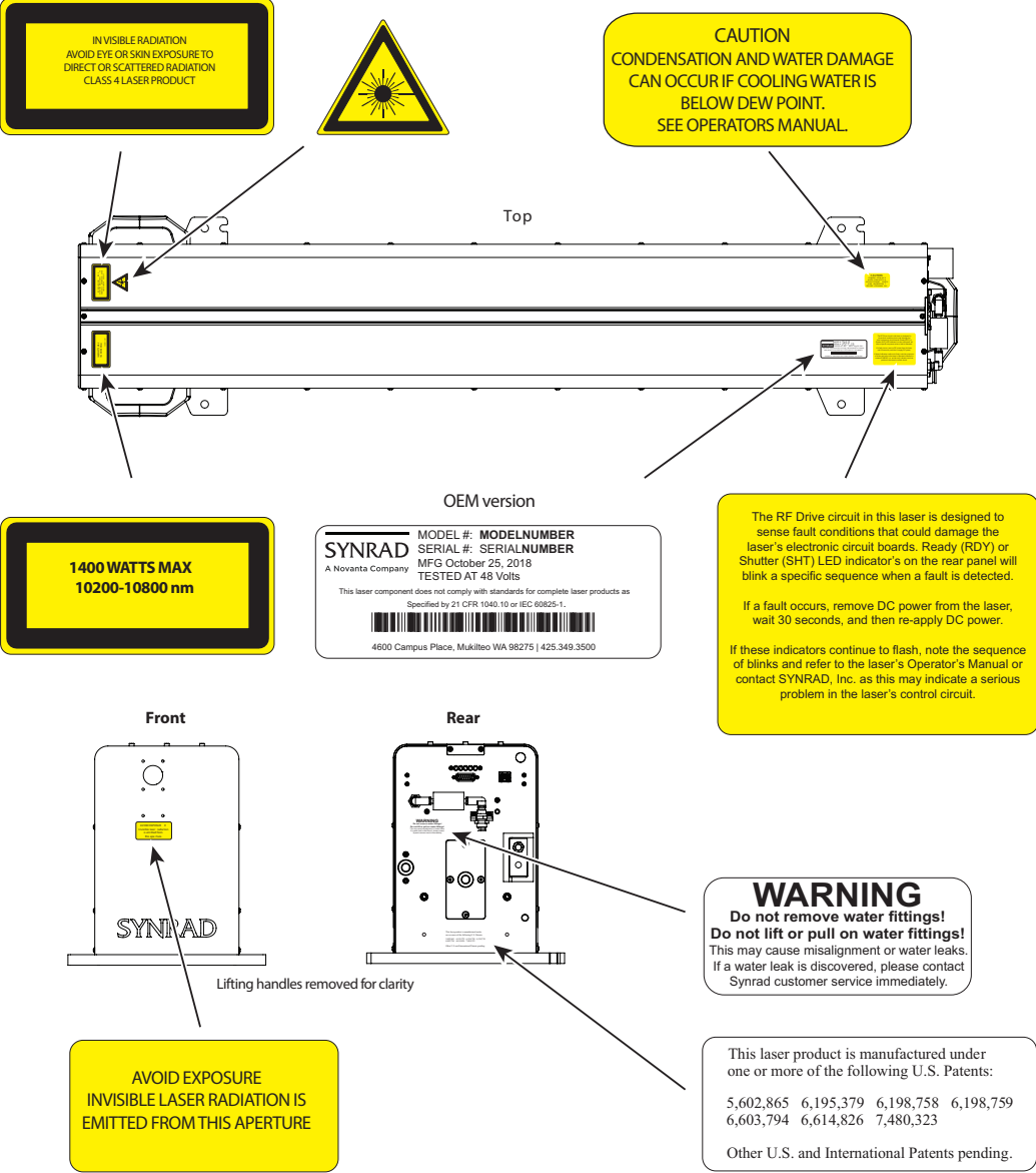
Figure 2-3 P400 hazard label locations.
