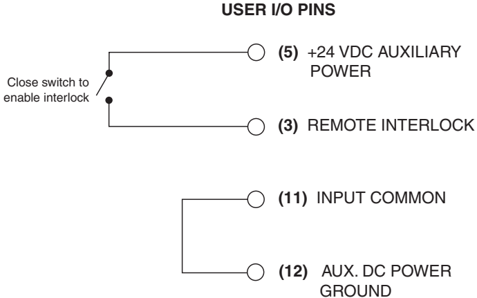
Figure 4-27 Customer-supplied interlock.
