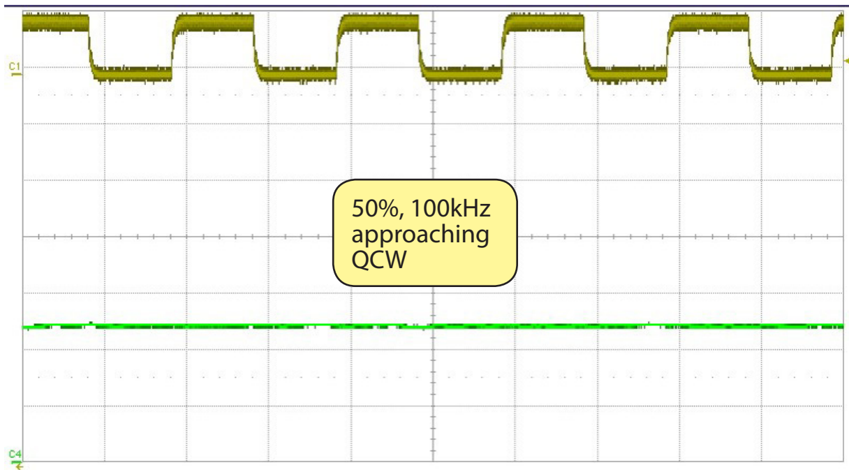
Figure 4-20 Representative output energy profile-50% duty cycle, 100 kHz, 5.0 \mu s/Dev timebase (approaching Quasi-Continuous Wave [QCW] output).
