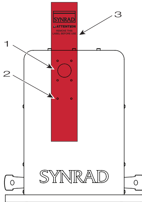
Figure 3-1 Pulstar p400 front panel controls and indicators.
