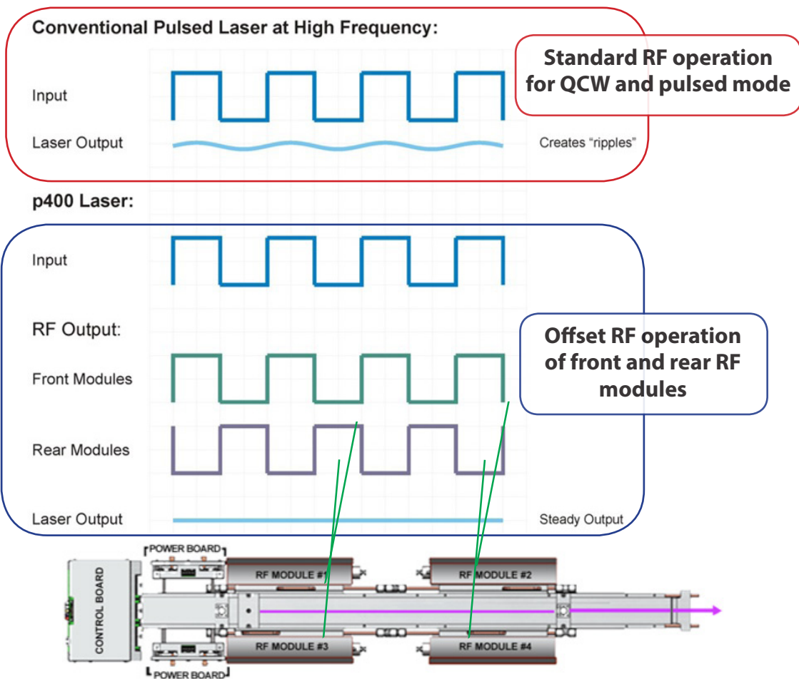
Figure 4-4 PWM command signal wave form (above) and Quasai Continuous Wave (QCW) explanation.
